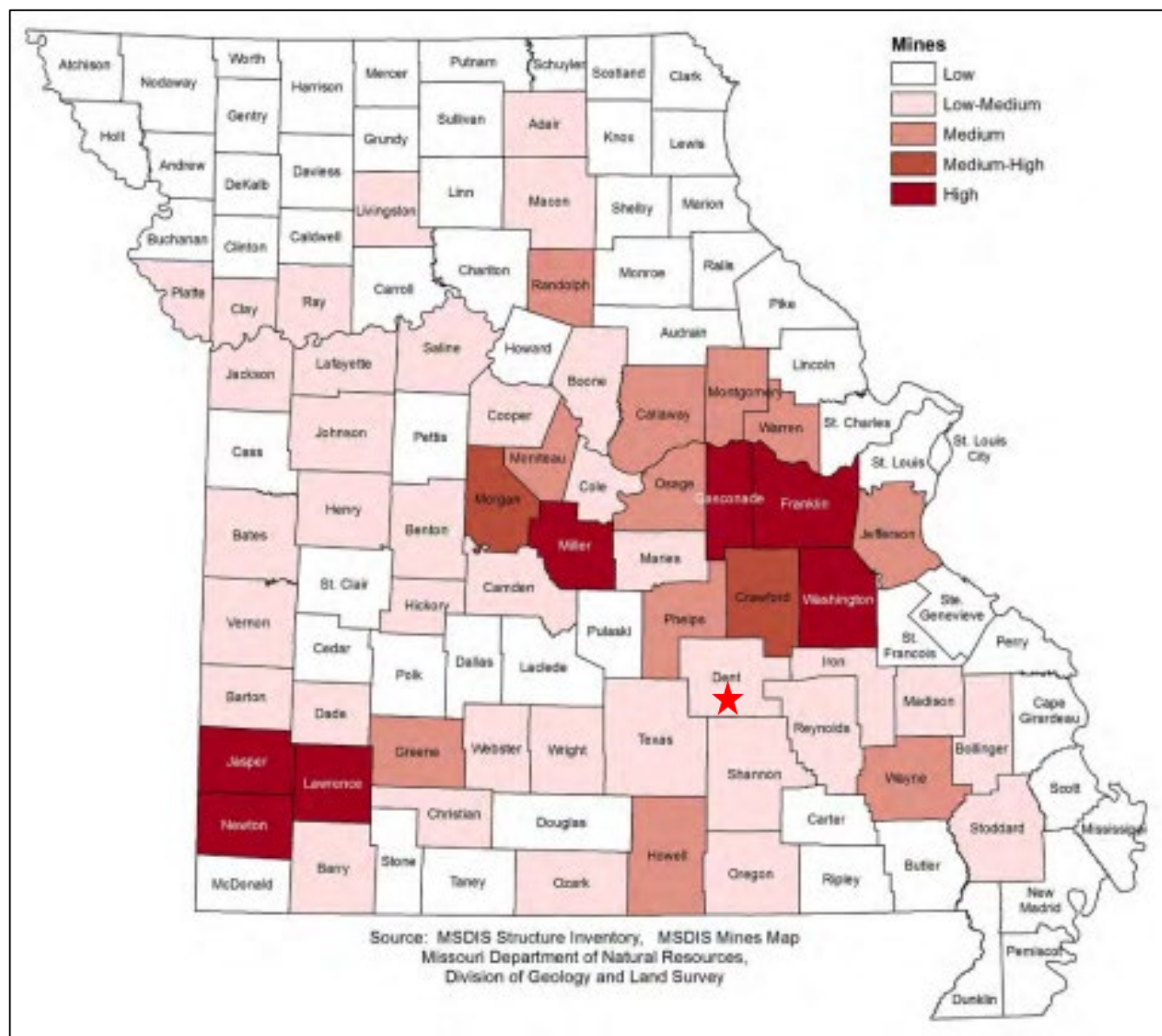
Figure 3.48. Mine Rating Value by County
