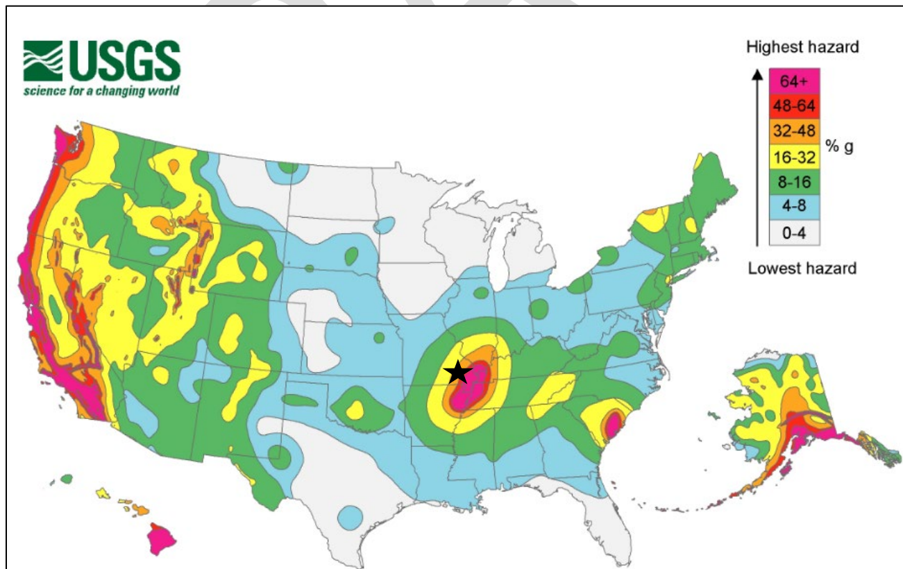
Figure 3.20. United States Seismic Hazard Map
