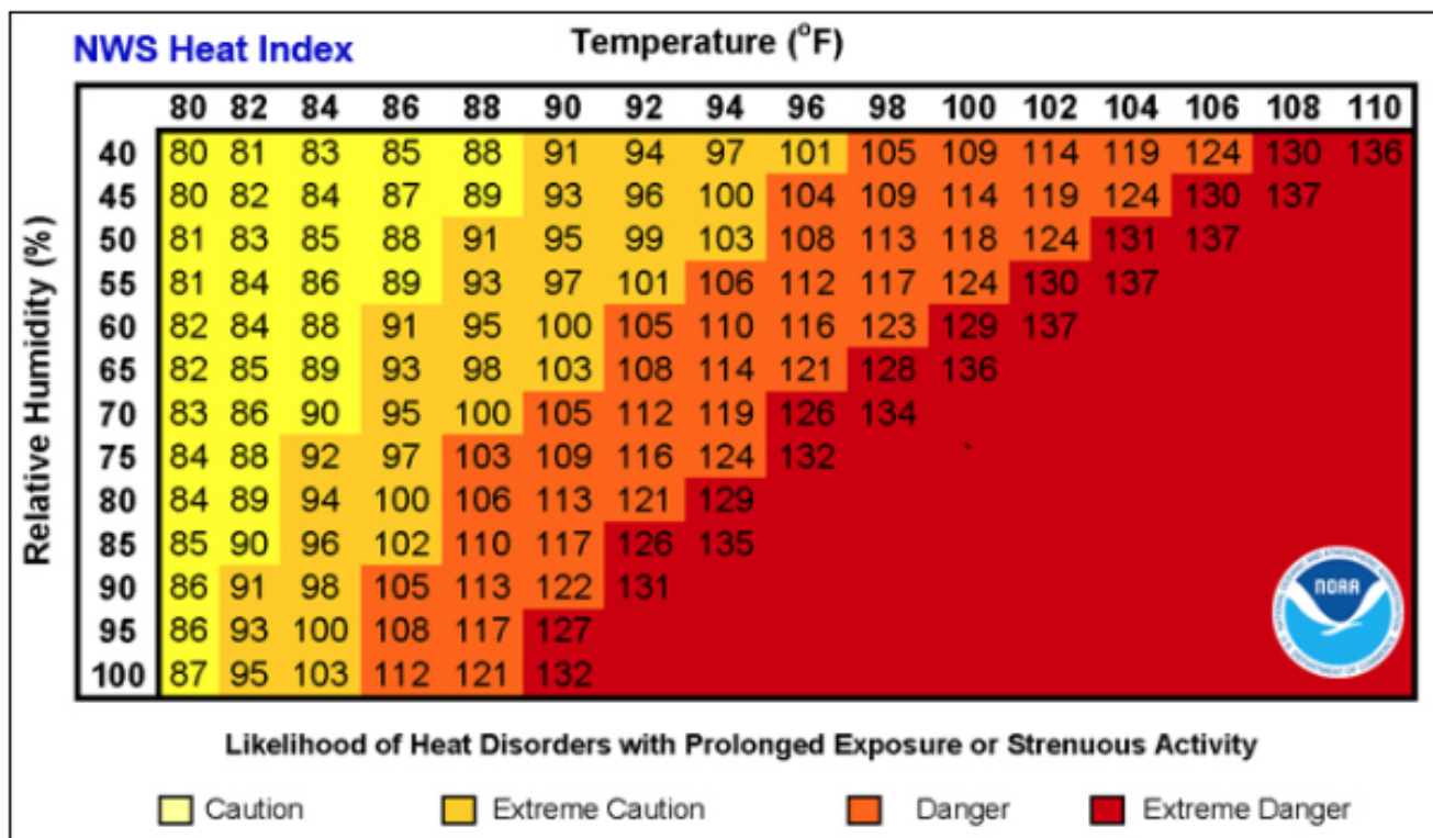
Figure 3.25. Heat Index (HI) Chart
