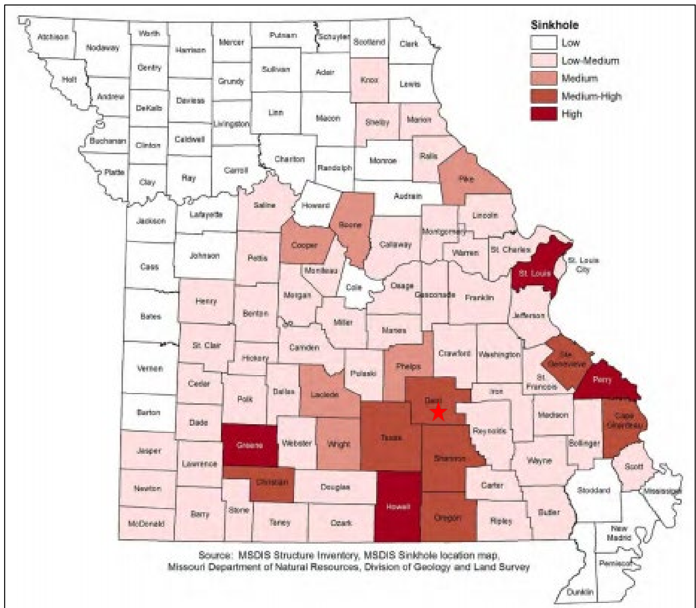
Figure 3.47. Sinkhole Rating Value by County
