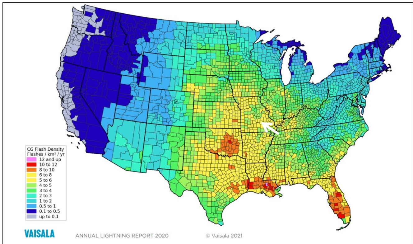
Figure 3.51. Location and Frequency of Lightning in Missouri
