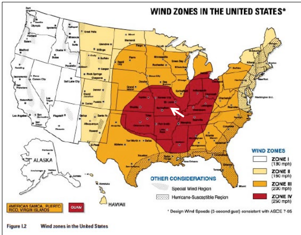
Figure 3.52. Wind Zones in the United States
