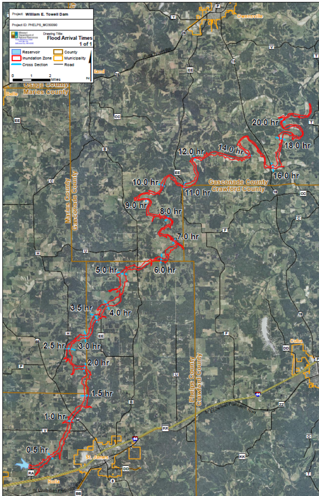
Figure 3.5. William E. Towell Dam Inundation Zone
