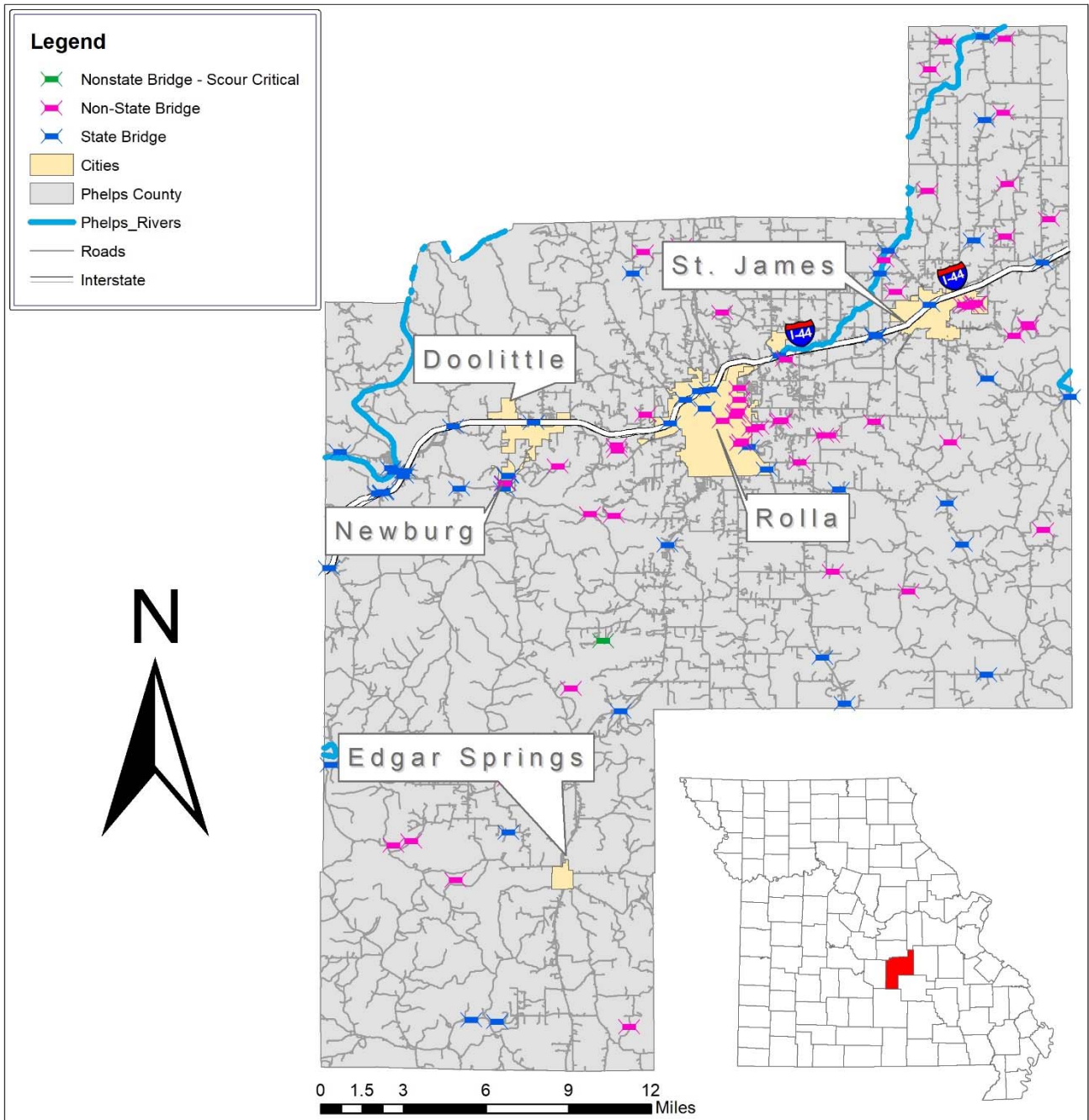
Figure 3.2. Phelps County Bridges
