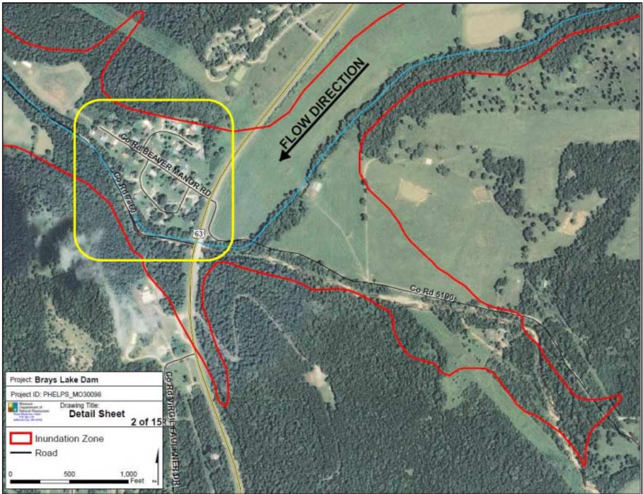
Figure 3.8. Brays Lake Dam Inundation Zone Continued
